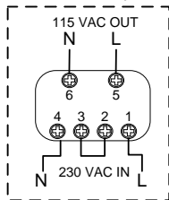
Power Transformer Connection for 230 VAC System
