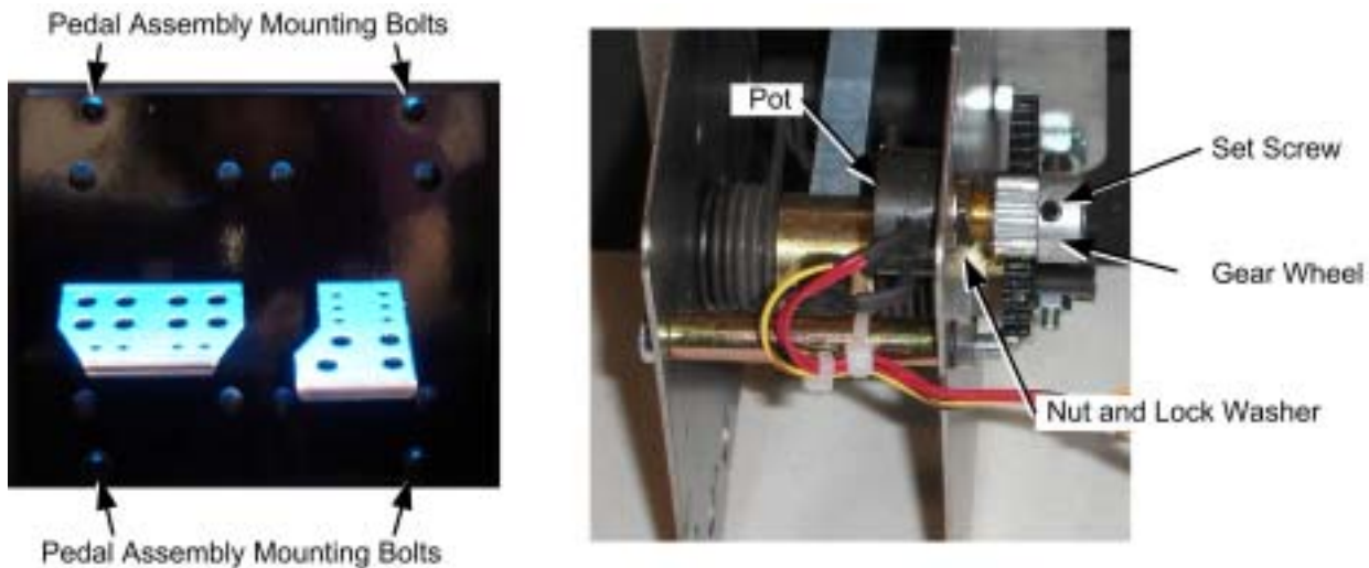
Figure 31. Pedal Assembly Details
