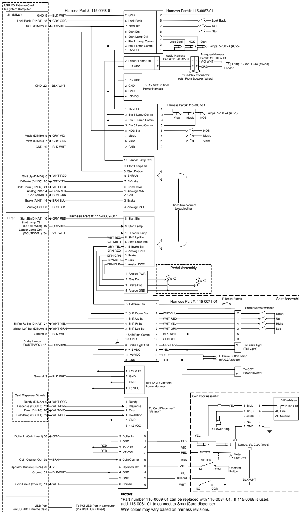
Figure 57. Detailed Wiring Diagram
