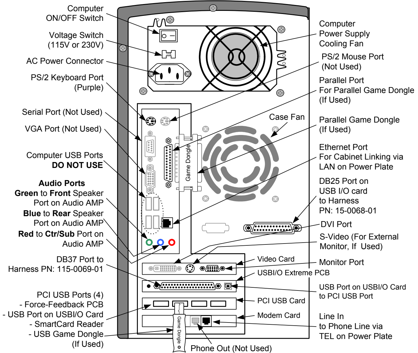
Figure 59. Computer Rear Panel Diagram
