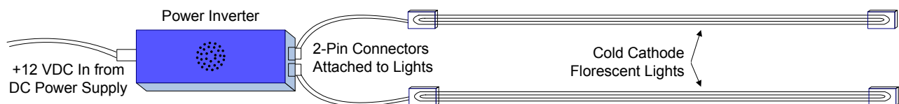
Figure 47. Cold Cathode Florescent Light Wiring
