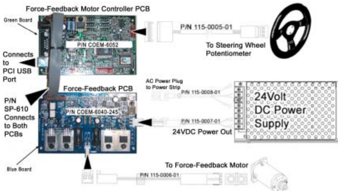
Figure 27. Force-Feedback Steering System Harnessing Diagram
