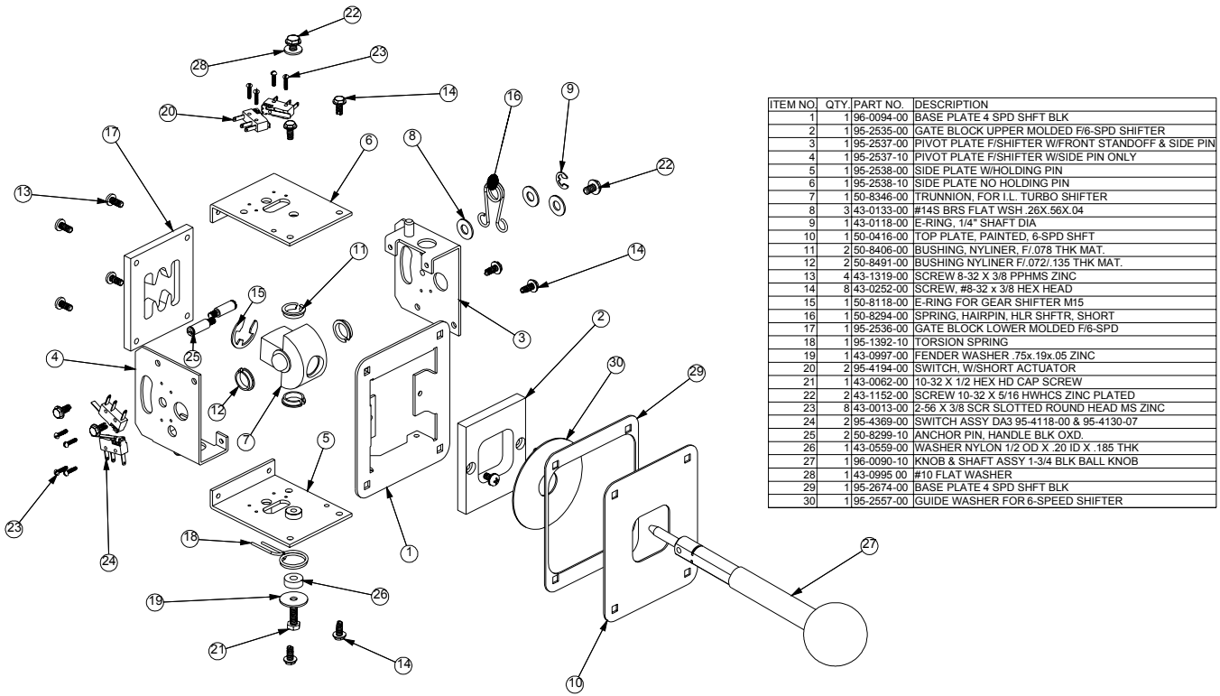
Figure 52. Six-Speed Shifter Exploded View and Parts
