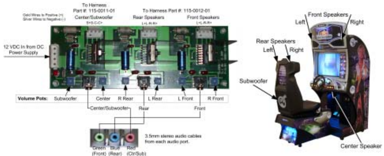
Figure 39. Audio Amp Connections, Volume Adjustment, and Speaker Location
