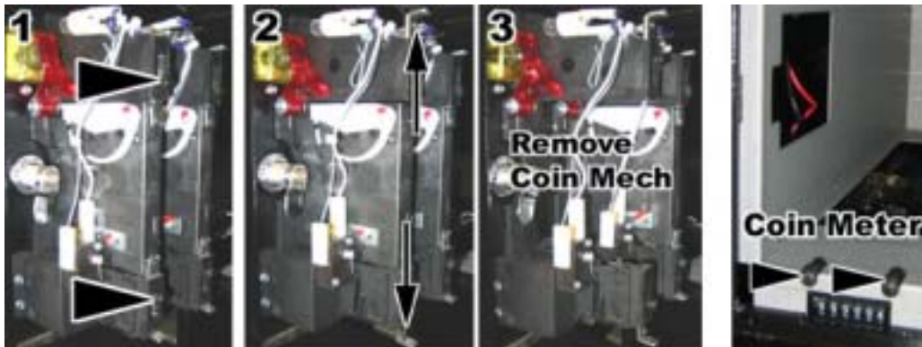
Figure 41. Servicing the Coin Mech and Coin Meter
