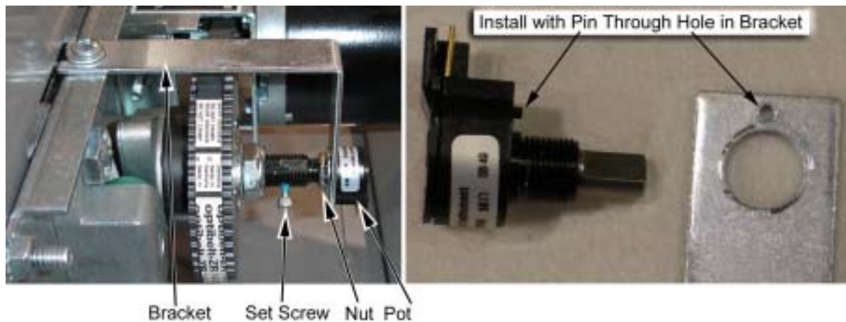
Figure 28. Replacing the 5 K \Omega Steering Pot
