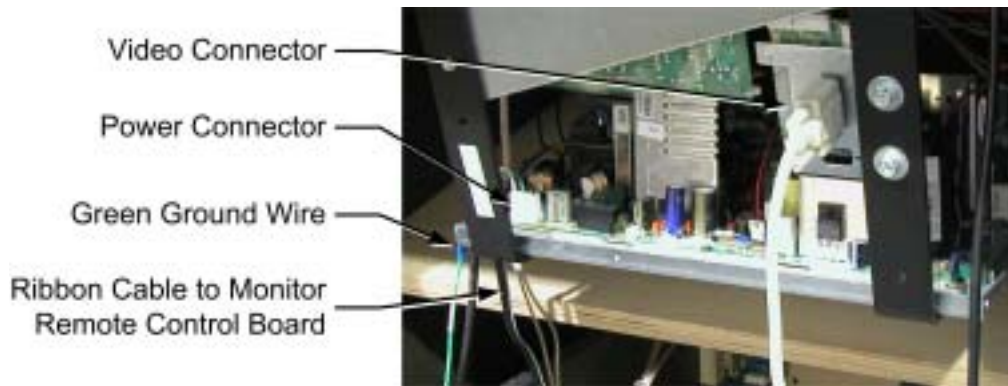
Figure 34. Cable Connections to the Monitor Chassis
