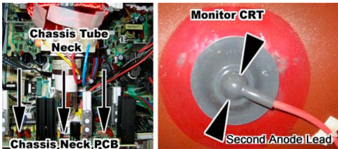
Figure 37. Disconnecting the Chassis Neck PCB and Second Anode Lead
