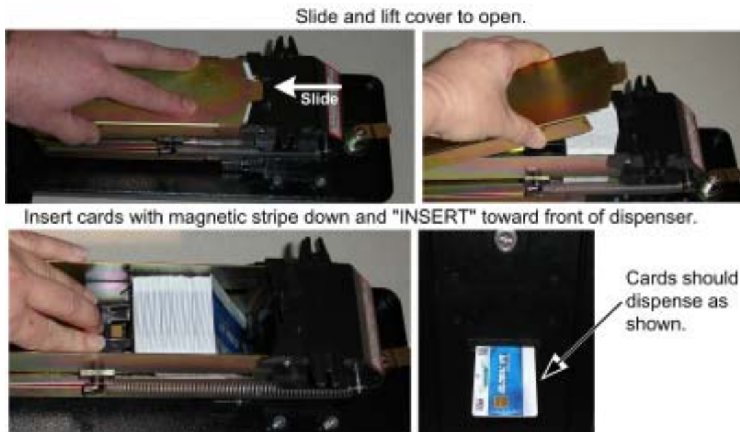
Figure 43. Filling the SmartCard Dispenser
