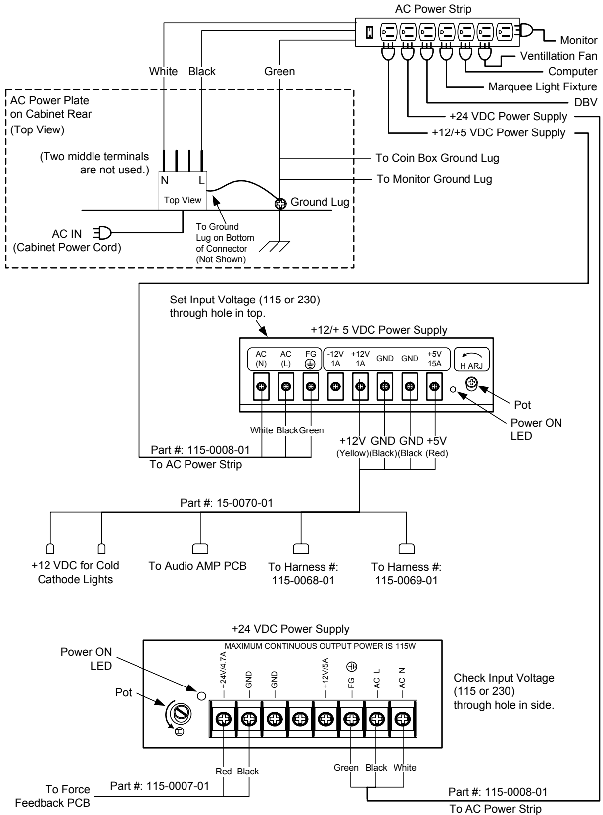
Figure 58. Power Distribution Diagram
