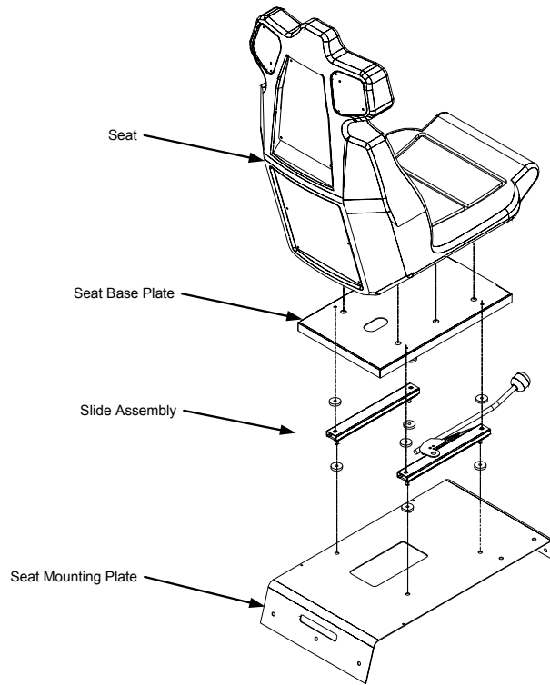
Figure 33. Seat Slide Assembly Replacement
