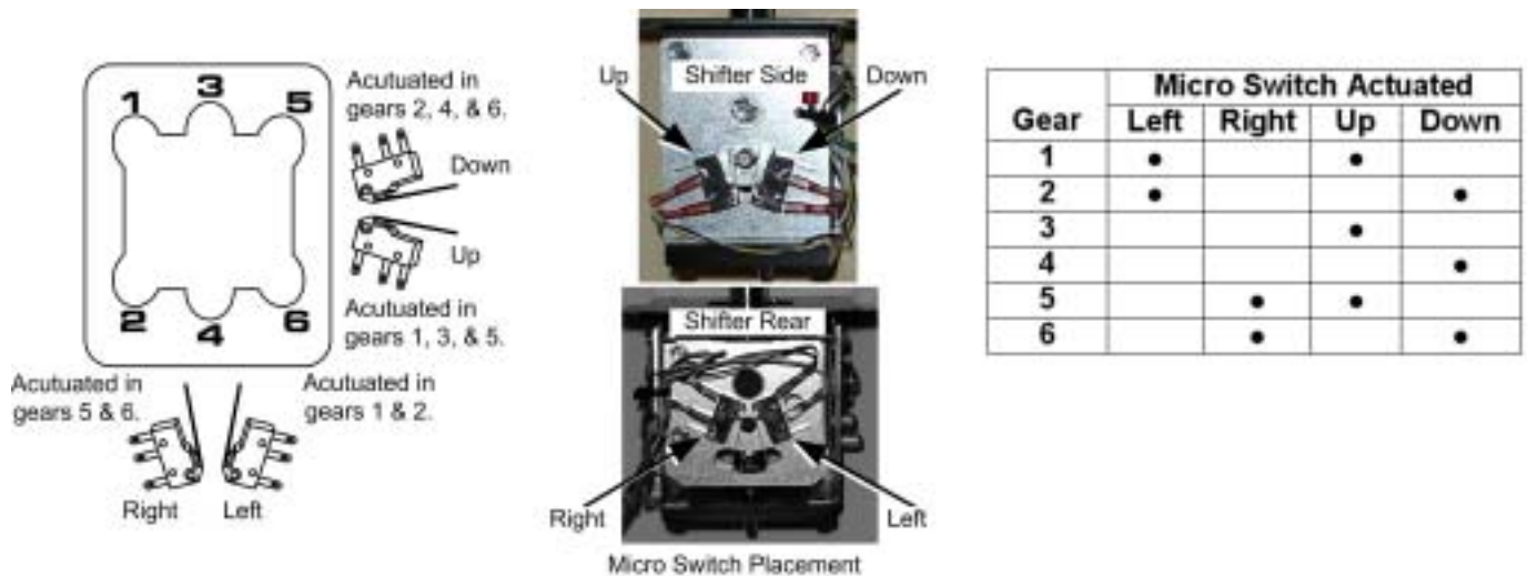
Figure 32. Shifter Pattern and Micro Switch Actuation
