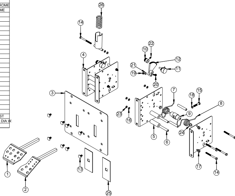
Figure 53. Pedal Assembly Exploded View and Parts
