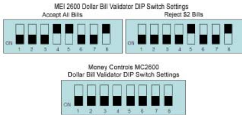
Figure 42. Dollar Bill Validator DIP Switch Settings
