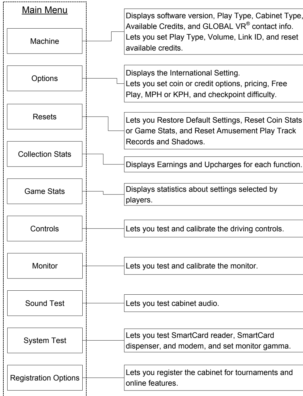
Figure 14. Game Operator Menu Flowchart
