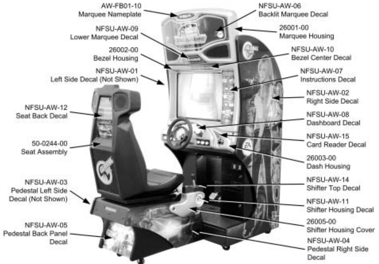
Figure 54. Artwork and Formed Plastic Part Numbers and Locations
