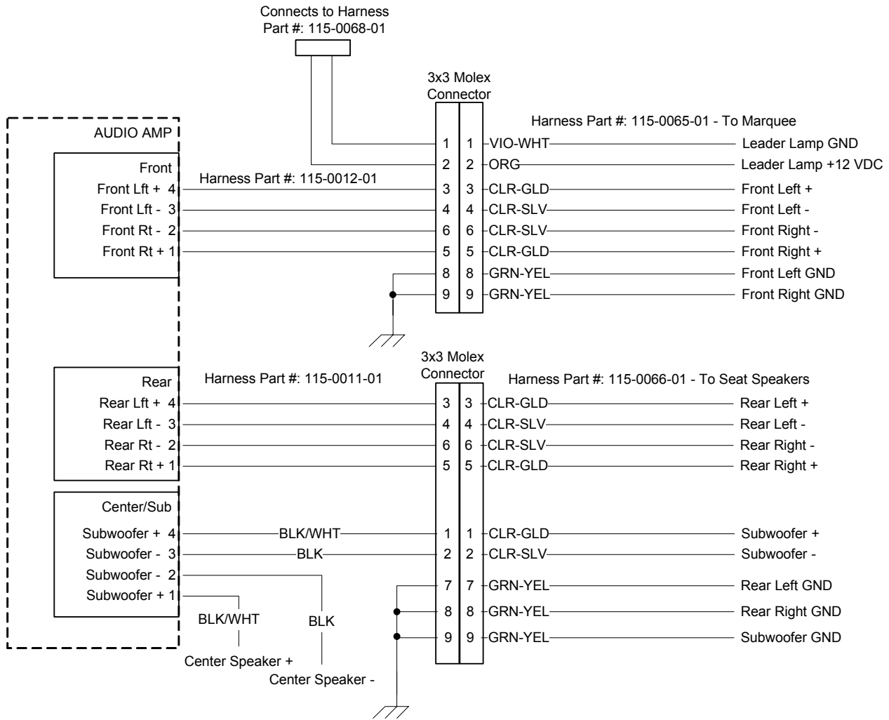
Figure 55. Audio Wiring
