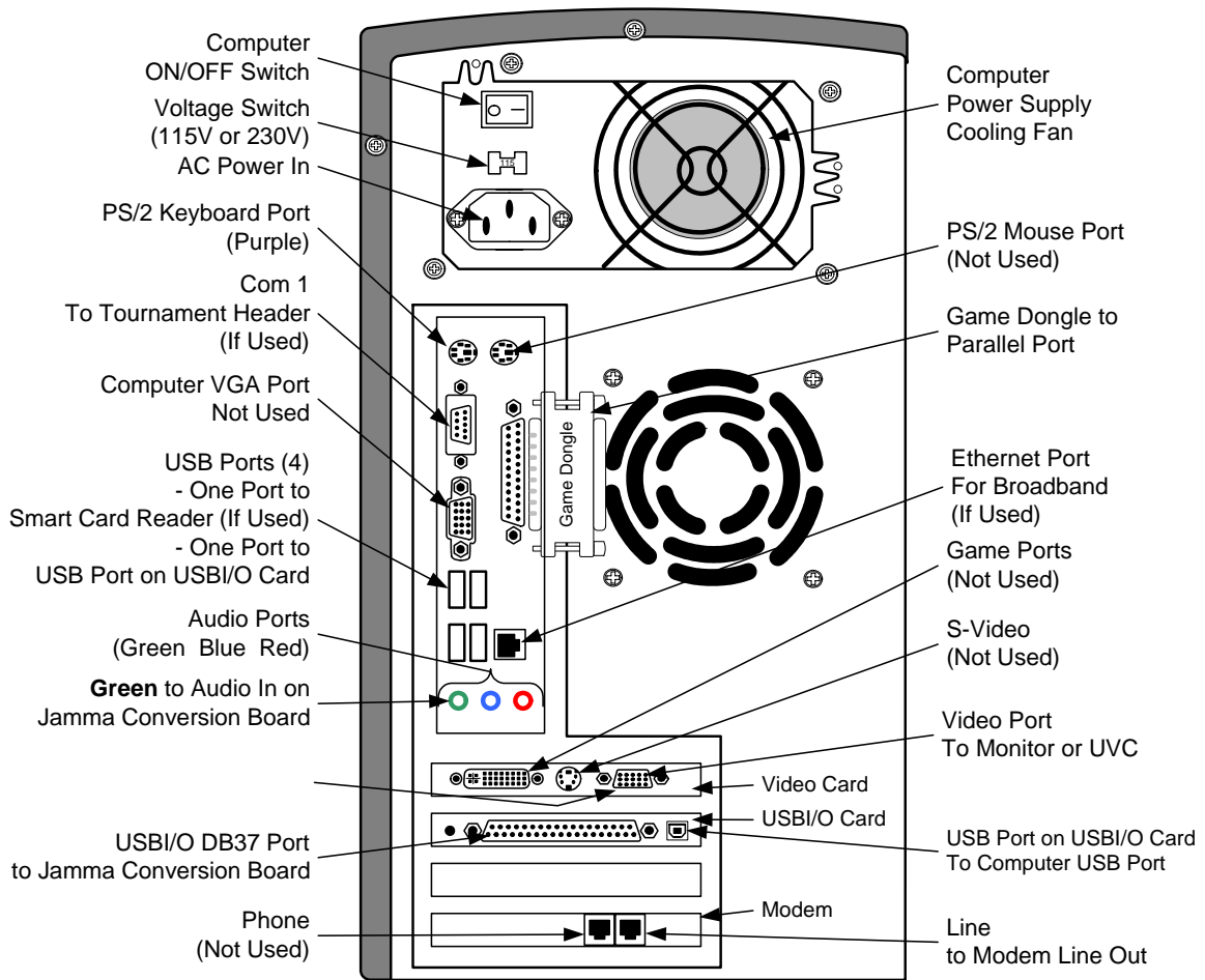
Figure 3. Computer Rear Connections
