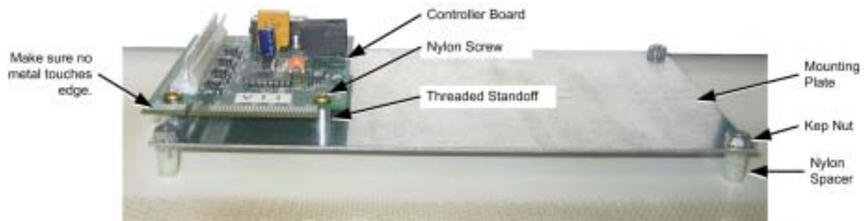
Figure 2. Mounting the Controller Board
