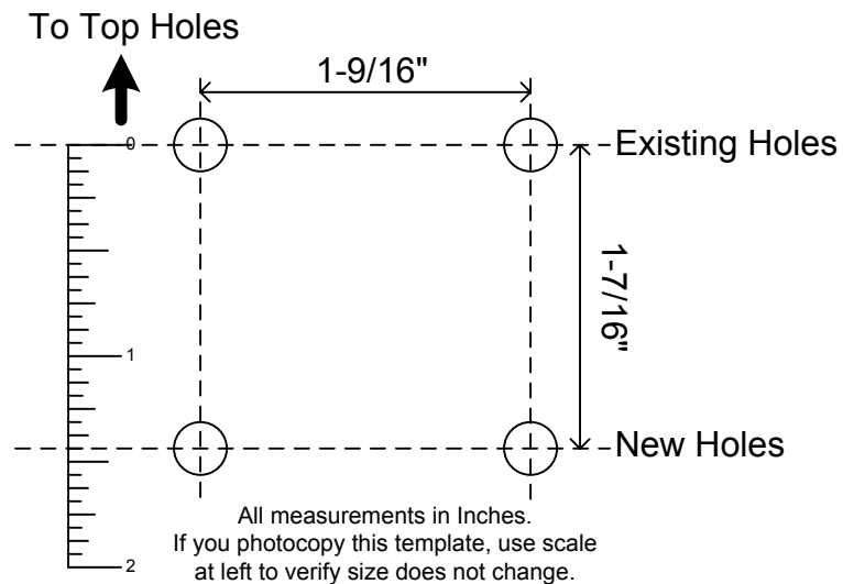
Template for Drilling Monitor Bracket Mounting Holes
