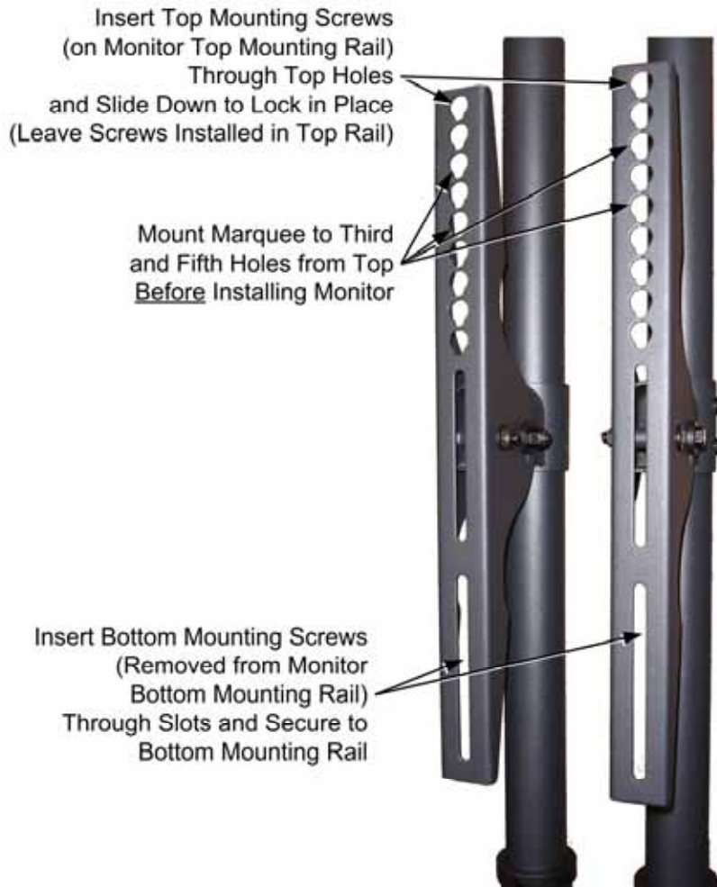
Figure 8. Vertical Rails on Monitor Stand
