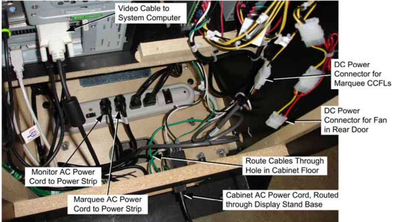
Figure 5. Cables Inside Cabinet
