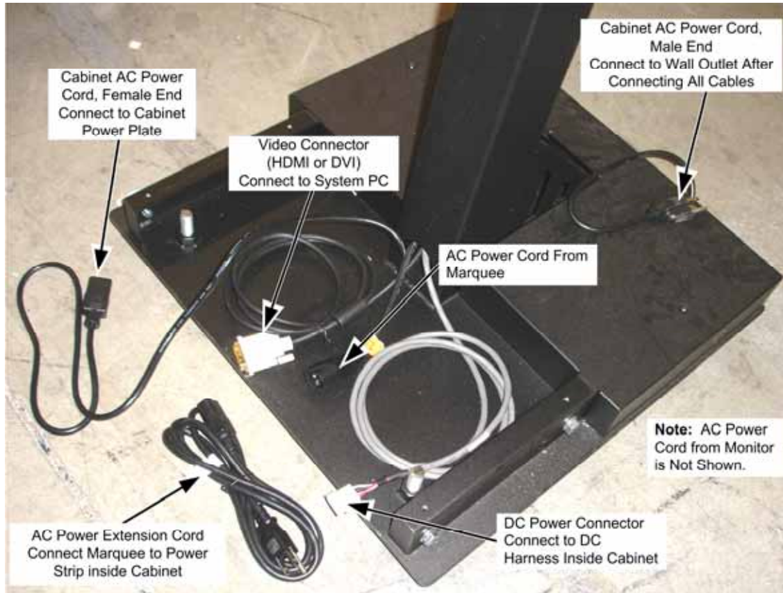
Figure 4. Cables in Display Stand Base
