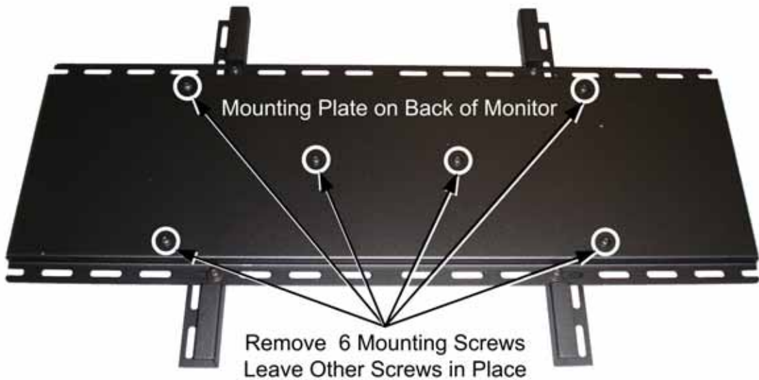
Figure 3. Mounting Plate on Back of Monitor
