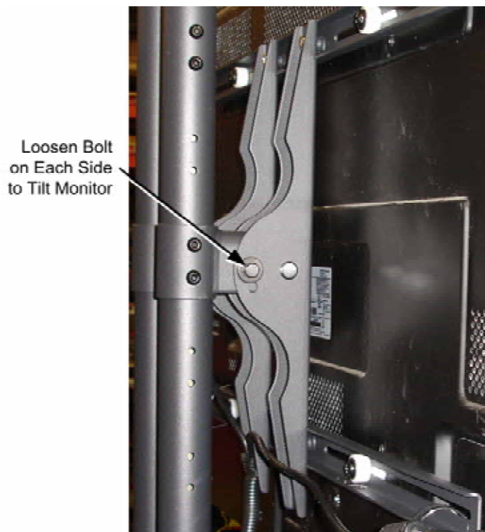
Figure 9. Tilting the Monitor
