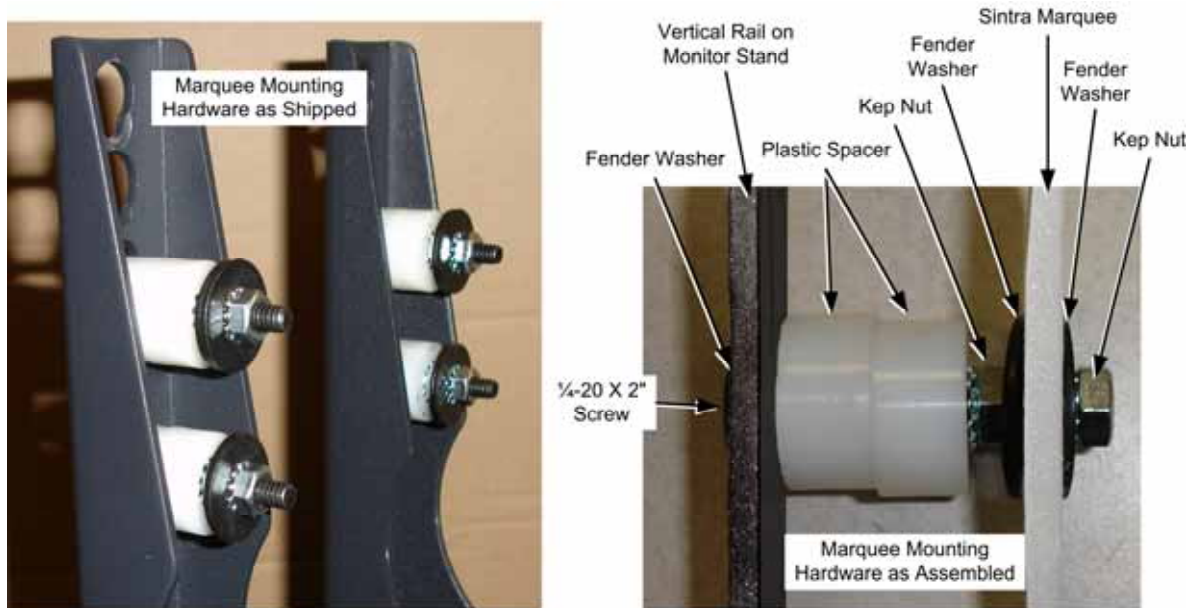
Figure 5. Marquee Mounting Hardware
